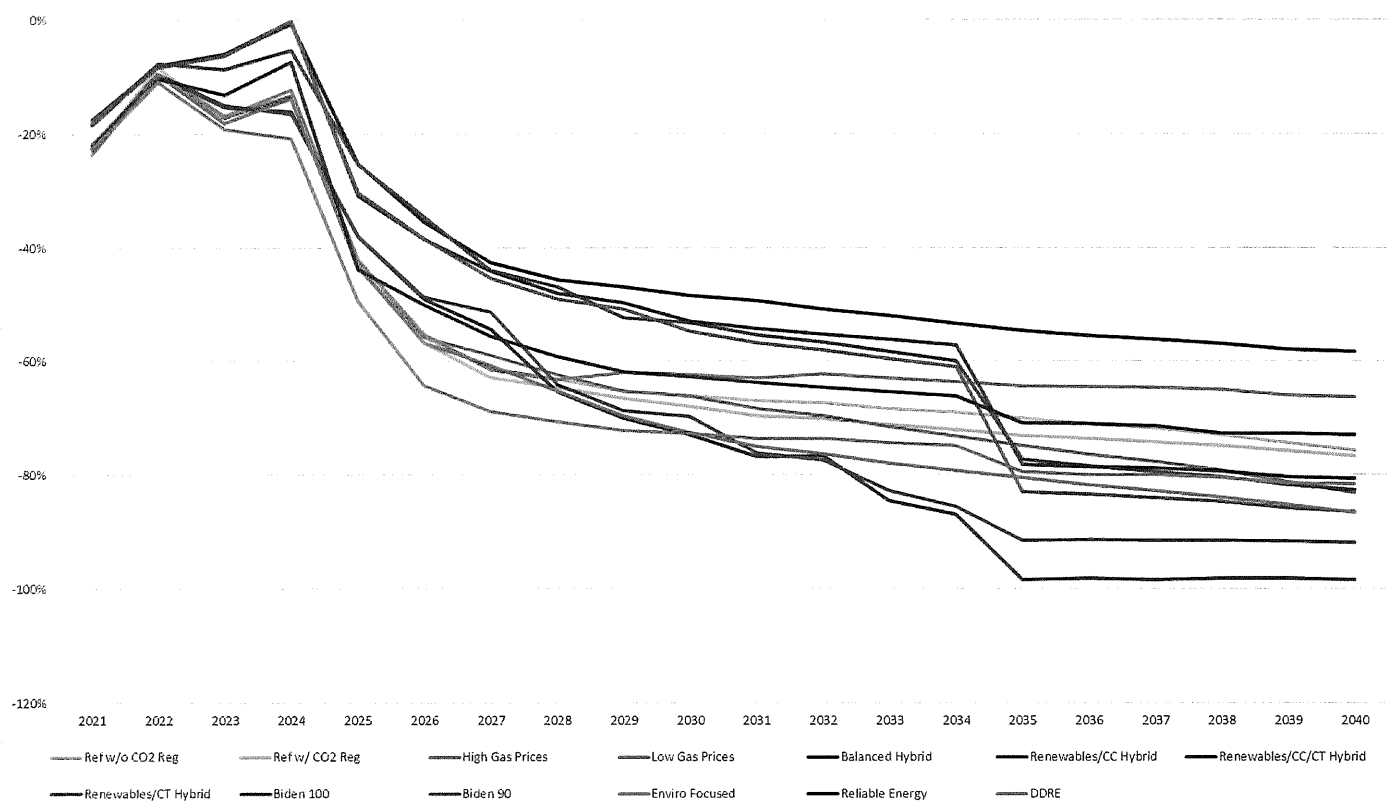
CO 2 Emissions by Portfolio in Ref w/ CO 2 Reg Scenario (% relative to 2005 Baseline)
