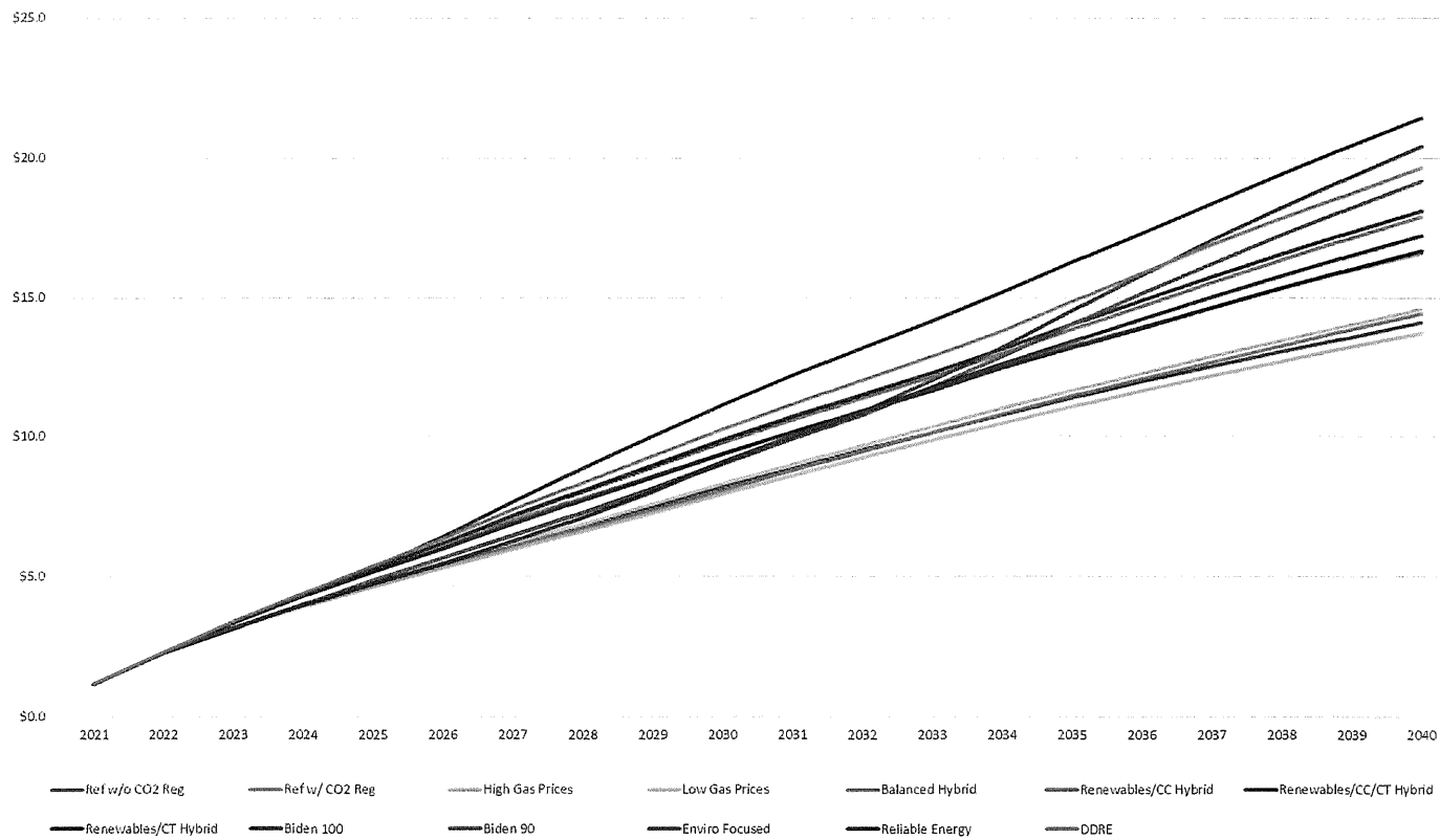
Portfolio PVRRs in Low Gas Scenario (in B$)
