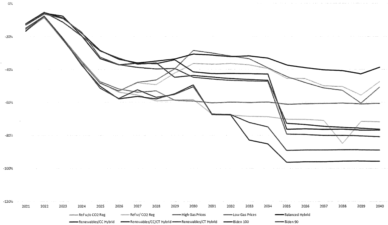
CO 2 Emissions by Portfolio in Low Gas Scenario (% relative to 2005 Baseline)
