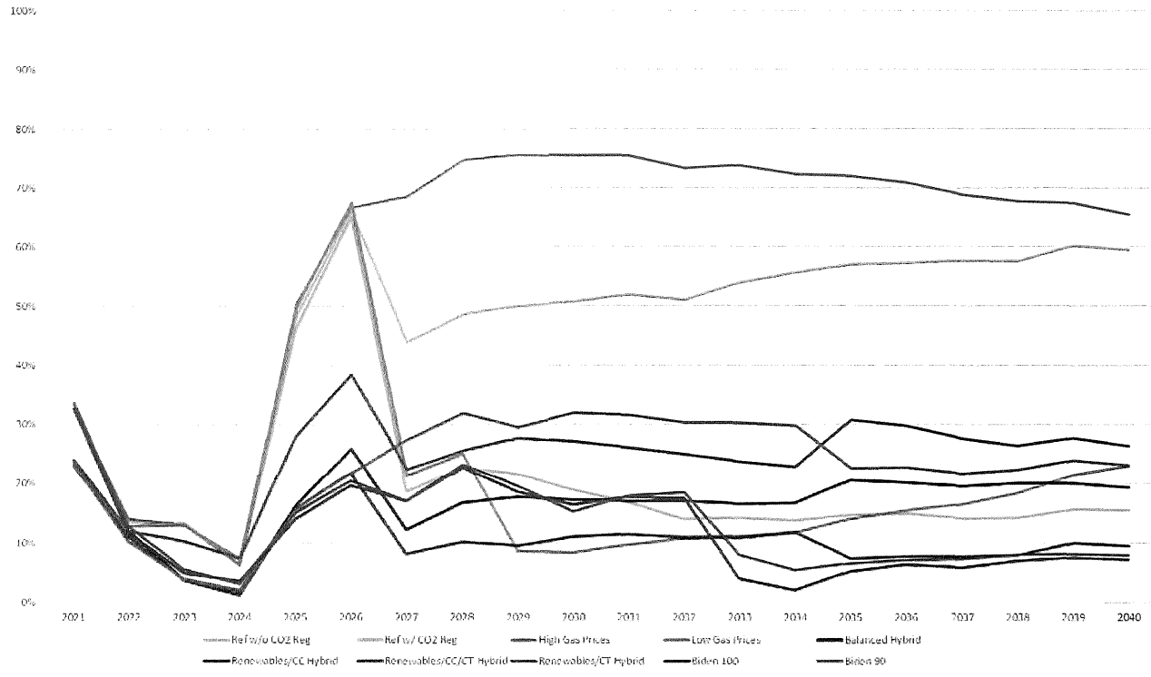
Market Purchases by Portfolio in Ref w/ CO 2 Reg Scenario (% of energy)
