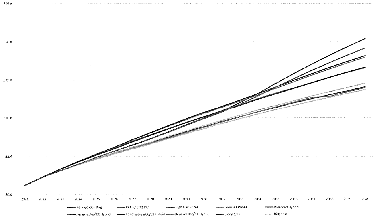
Portfolio PVRRs in Low Gas Scenario (in $)
