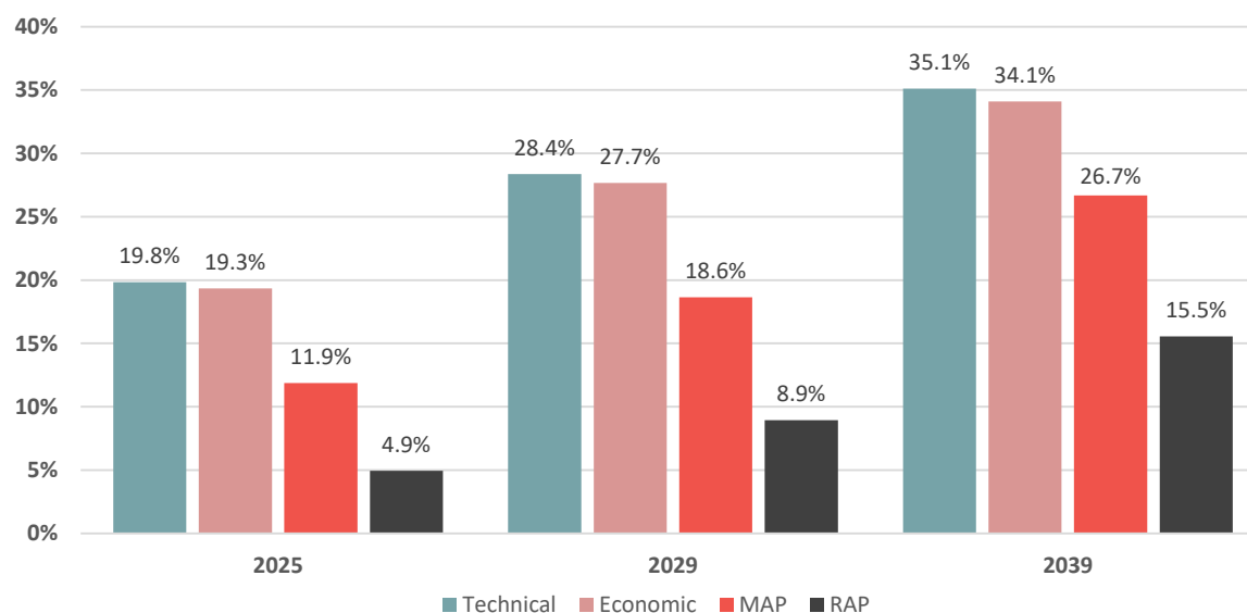
FIGURE 5-1 COMMERCIAL NATURAL GAS ENERGY CUMULATIVE ANNUAL POTENTIAL (AS A % OF COMMERCIAL SALES)
