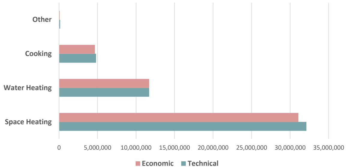
FIGURE 5-2 6-YEAR TECHNICAL & ECONOMIC COMMERCIAL NATURAL GAS POTENTIAL – BY END-USE
