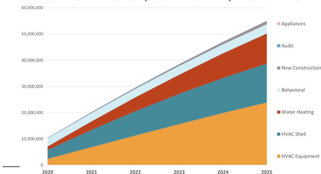
FIGURE 4-4 RESIDENTIAL NATURAL GAS (CUMULATIVE ANNUAL THERMS) RAP POTENTIAL BY END-USE
