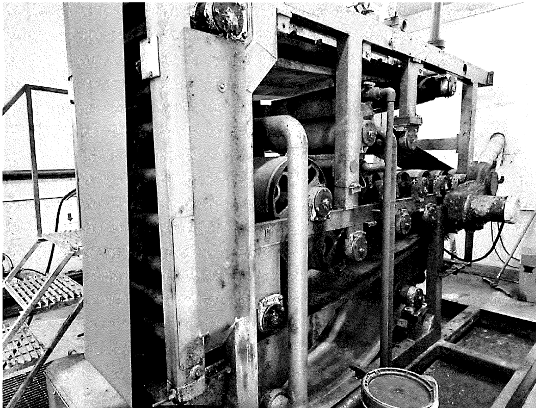
PHOTO 18: SLUDGE PRESS
