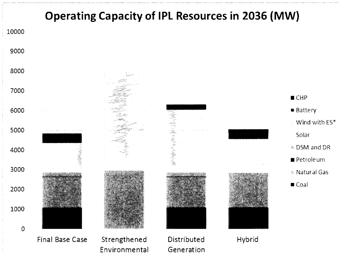
Figure 8.67 – Operating Capacity in 2036 with Hybrid Portfolio
