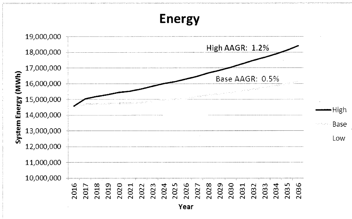
Figure 7.6 – IPL Peak and Energy Load Forecast
