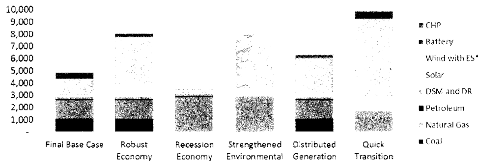
Figure 4 - Candidate Resource Portfolios (MW in 2036)
