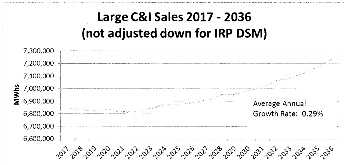
Figure 4.17 – Large C&I Sales
