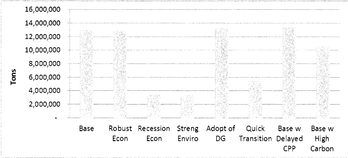
Figure 8.54 – Results CO 2 emissions by Scenario
