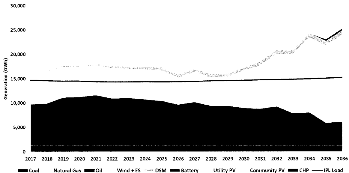
Figure 8.10 – Robust Economy Energy
