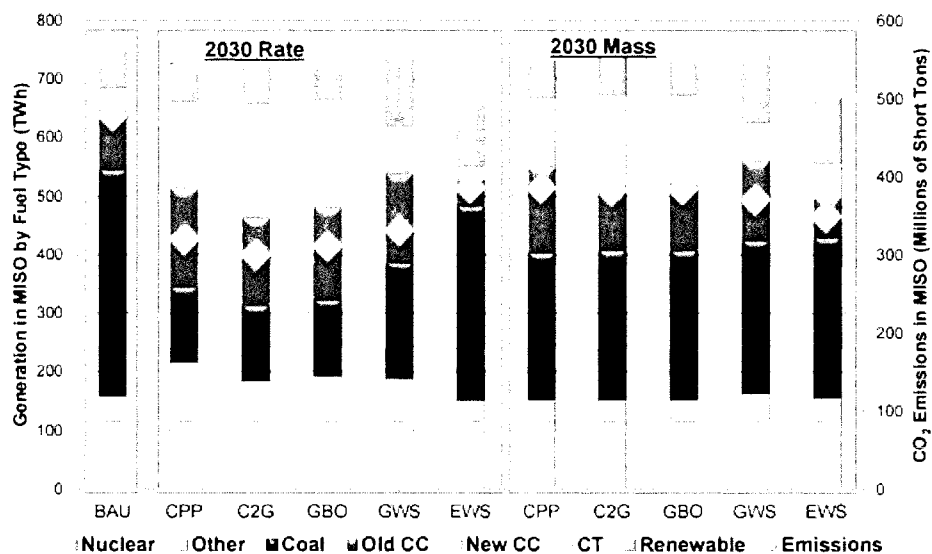
Figure 5.13 – 2030 Generation in MISO by Fuel Type across MISO CPP Scenarios
