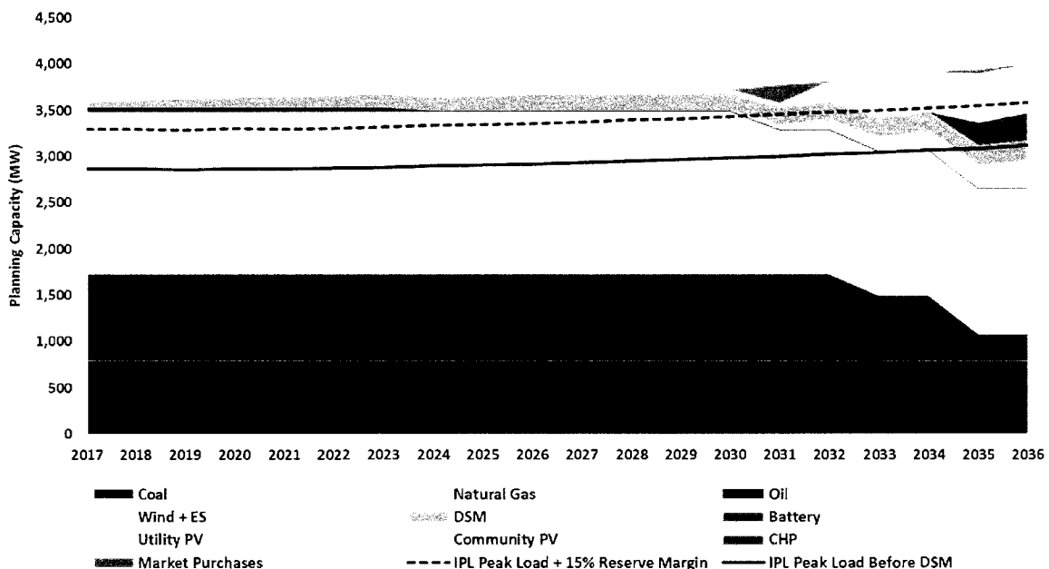
Figure 8.8 – Robust Economy Planning Capacity
